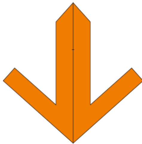
cub tetrakis
