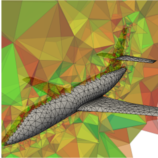
Mesh for 3D Finite Element computations
