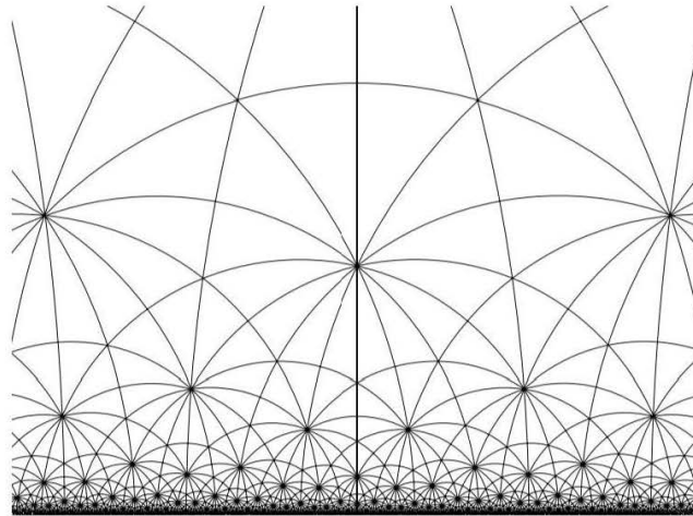
Tiling by repeated reflections
